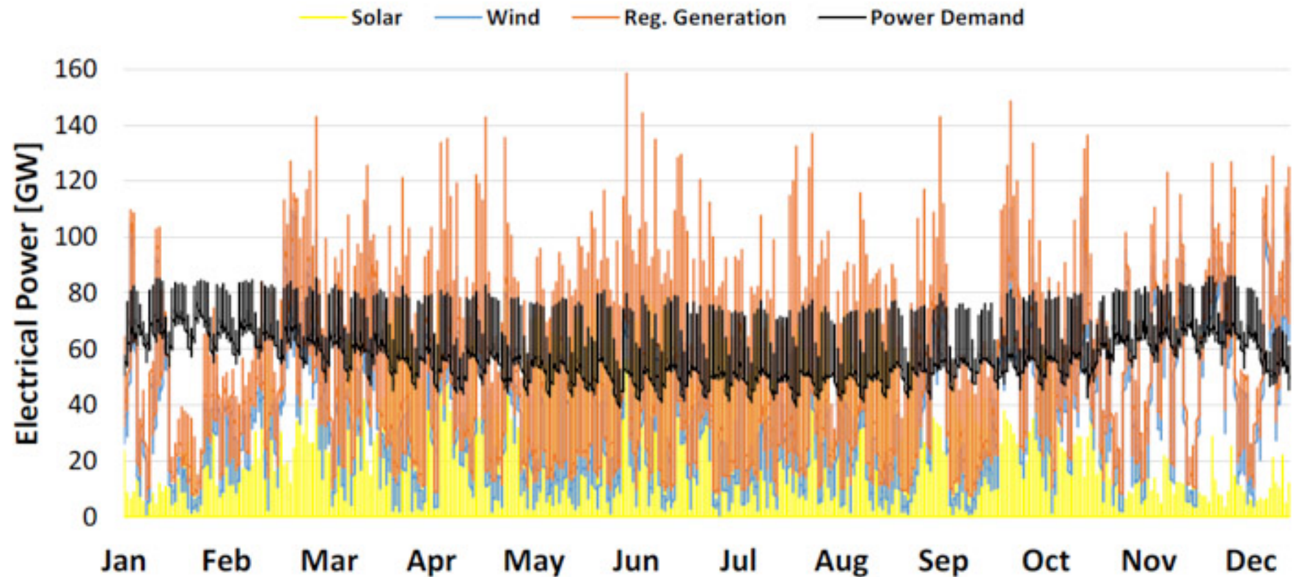
Fig. 5 Evolution of selected electricity sources P_{ijk} over j hours ( i=1 wind, i=3 solar/photovoltaic, sum of i=1-4 ; j within the range 1:8760; k=2035 ): simulated performance 2035, based on 2017 analysis; electric power demand D_{jk} without BEV
